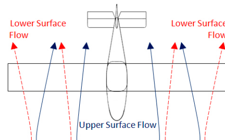
Fig. 2. Tip flow for an aircraft wing when producing lift
