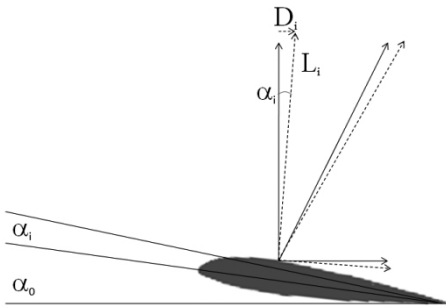
Fig. 4. Induced flow at the total angle of attack requires the aerodynamic reaction force to be longer, increasing the length of the relative vertical component
