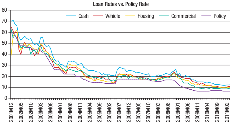
Fig. 1. Loan rates and policy rate in Turkey during 2001M12–2011M04
