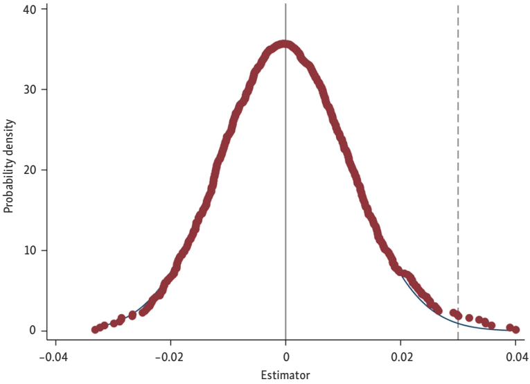
Figure 4. Placebo test
